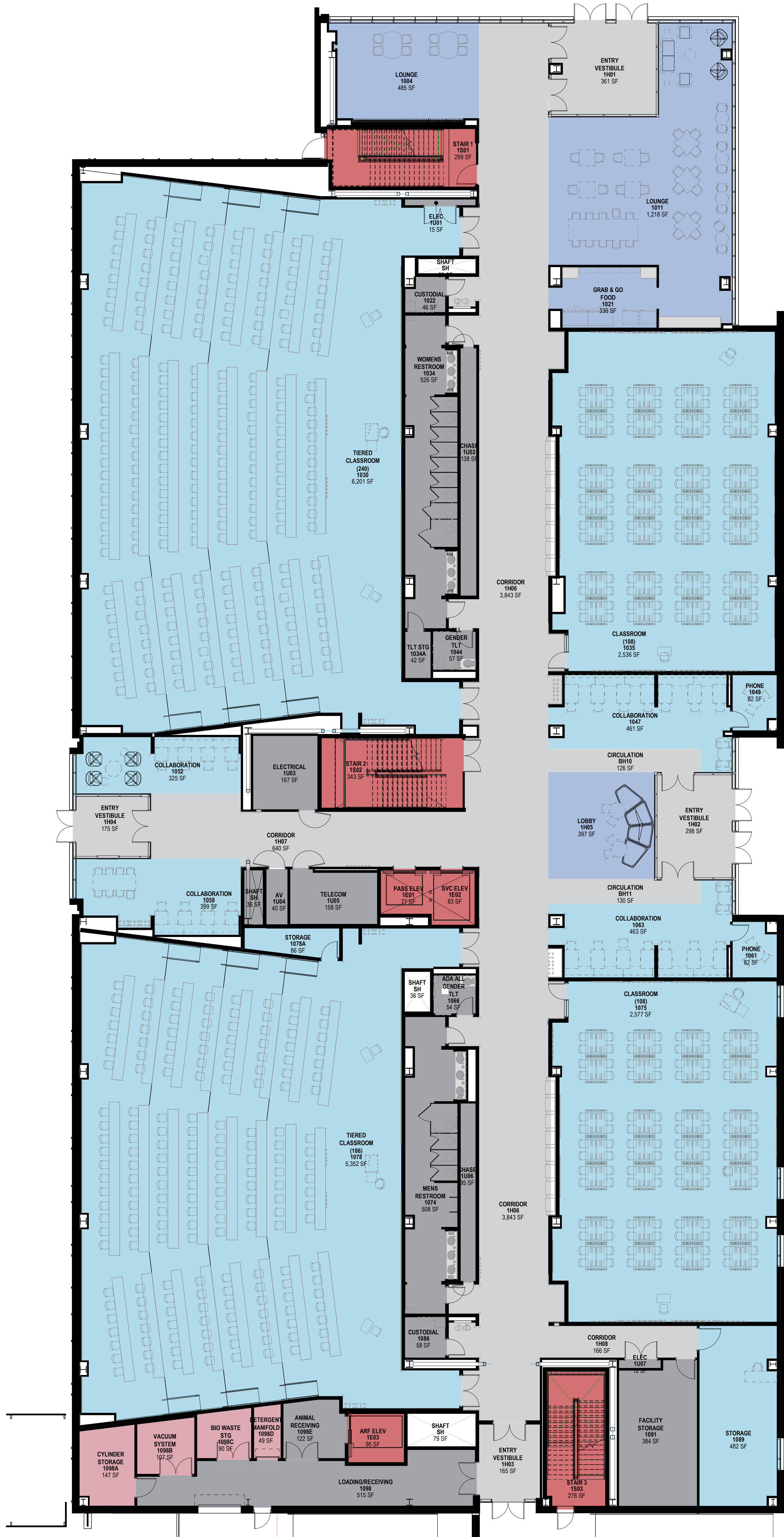
01 - FIRST LEVEL - DEPARTMENT PLAN 3/32" = 1'-0"
